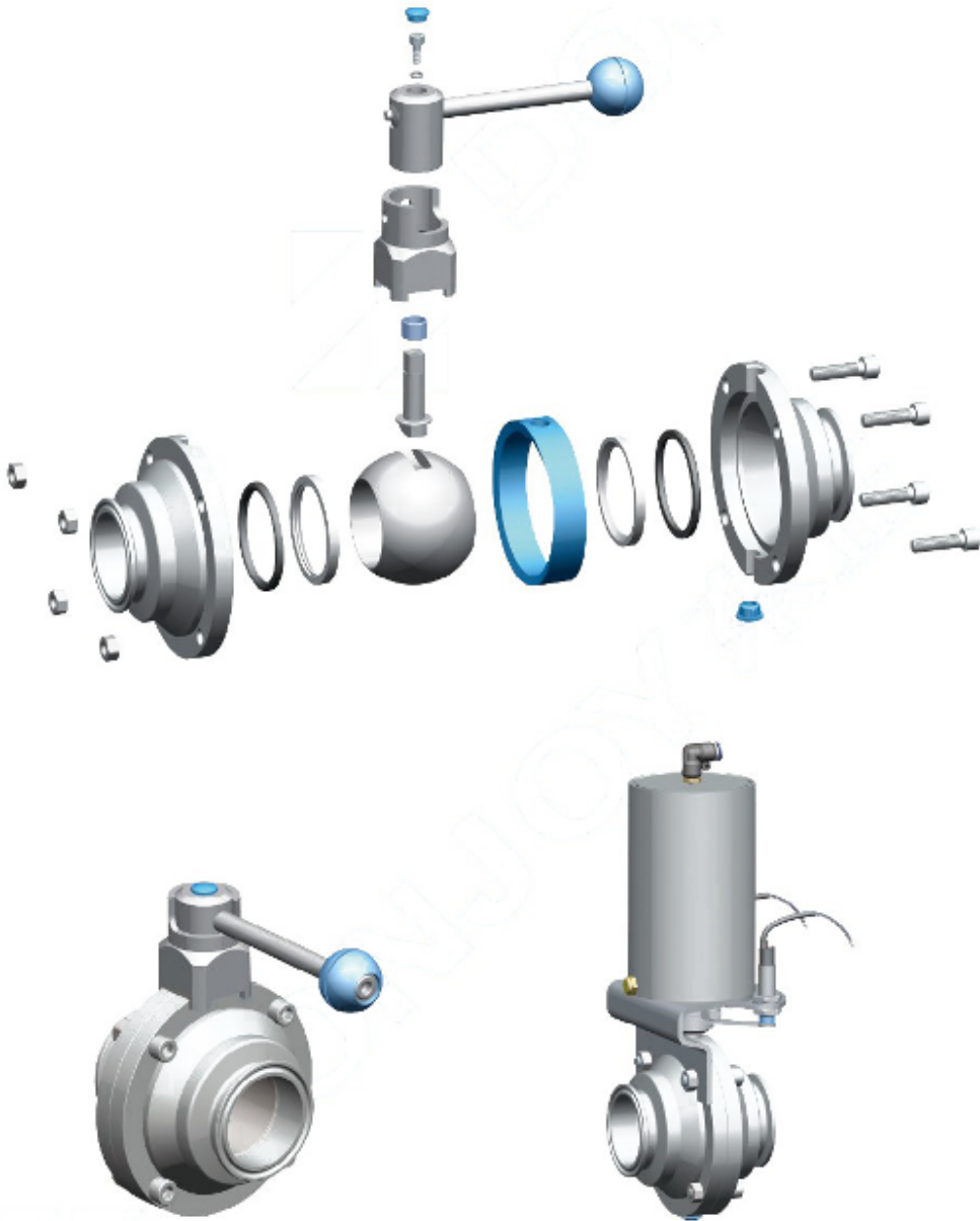
Butterfly-type ball valve
