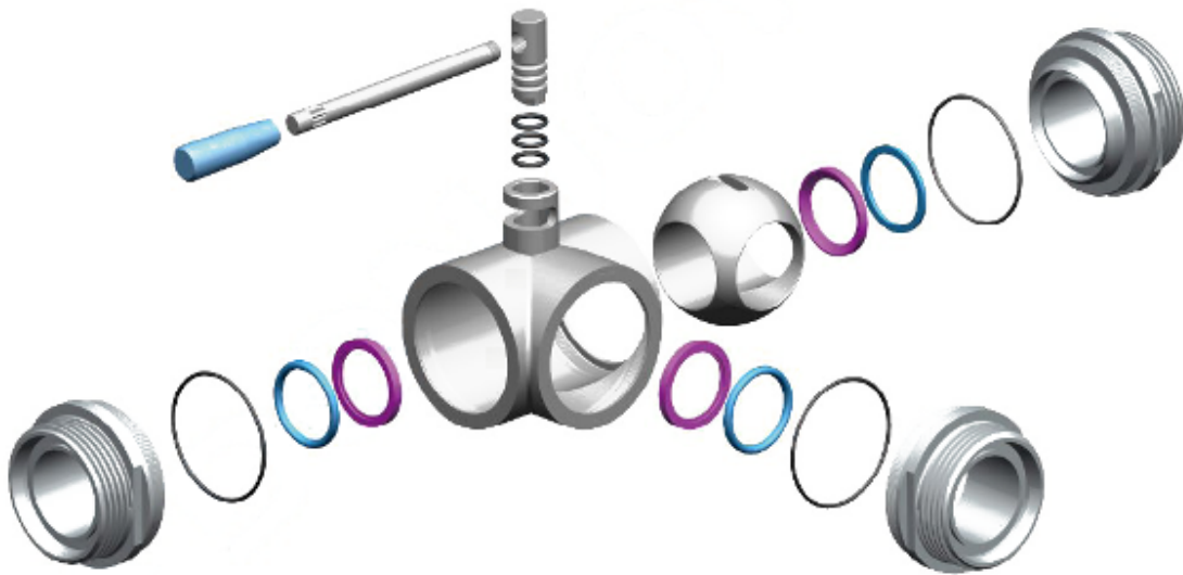
Three-piece ball valve
